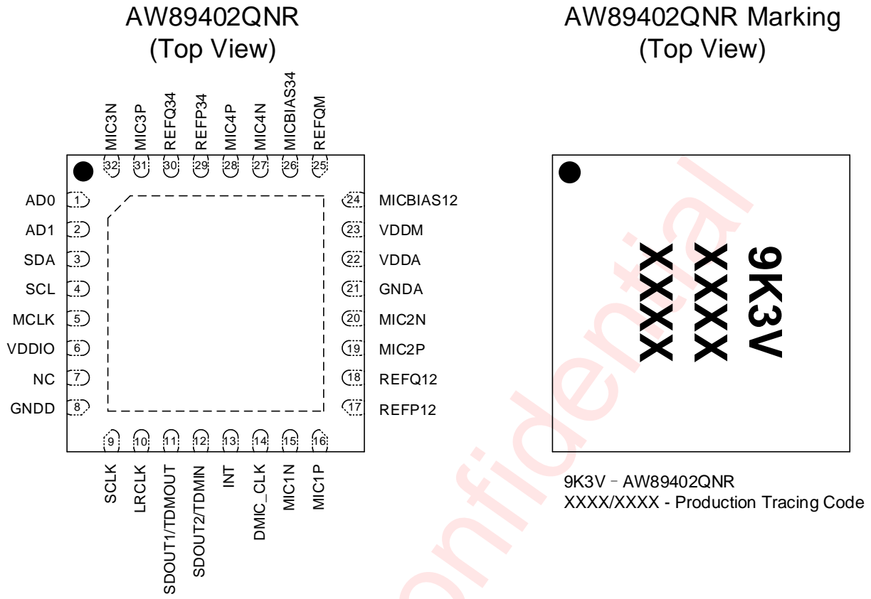
Figure 3 AW89402 pin diagram top view and device marking
