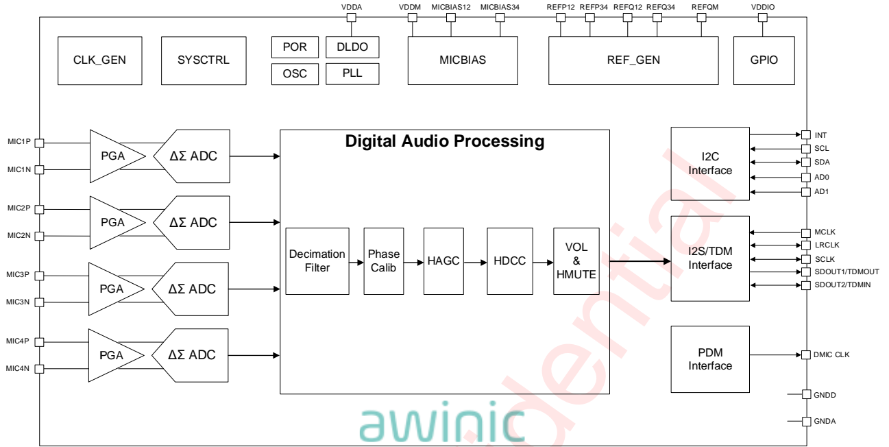
Figure 1 AW89402 Functional Diagram
