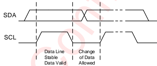
Figure 14 Data Validation Diagram
