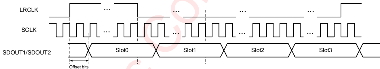
Figure 11 TDM Timing
