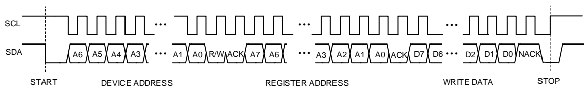
Figure 17 I 2 C Write Byte Cycle
