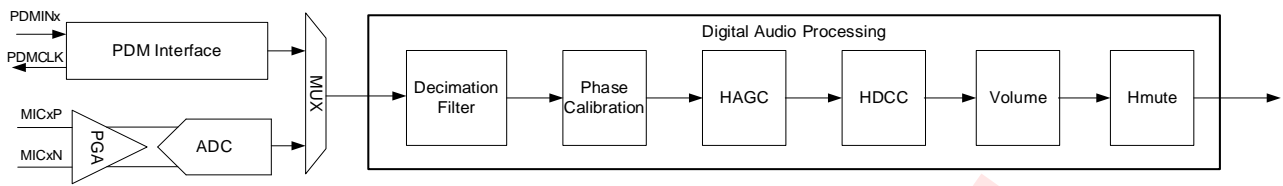
Figure 12 Block Diagram of DAP
