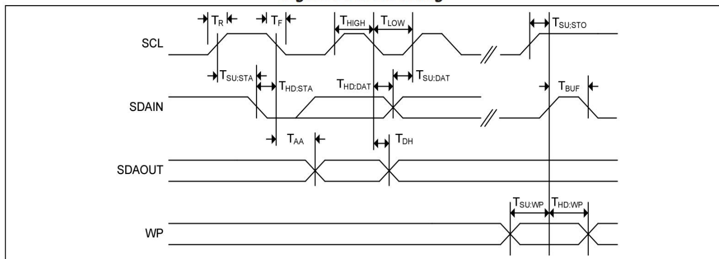
Figure 1-11. Bus Timing
