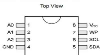
8-Pin SOIC/SOP and TSSOP /DIP
