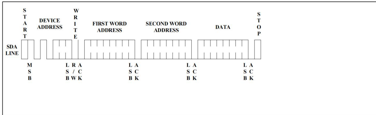
Figure 6. Byte Write
