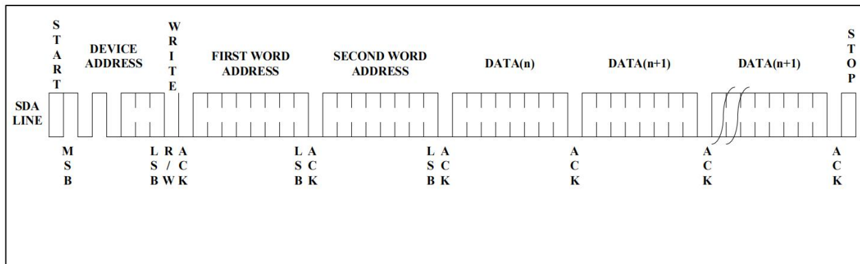
Figure 7. Page Write
