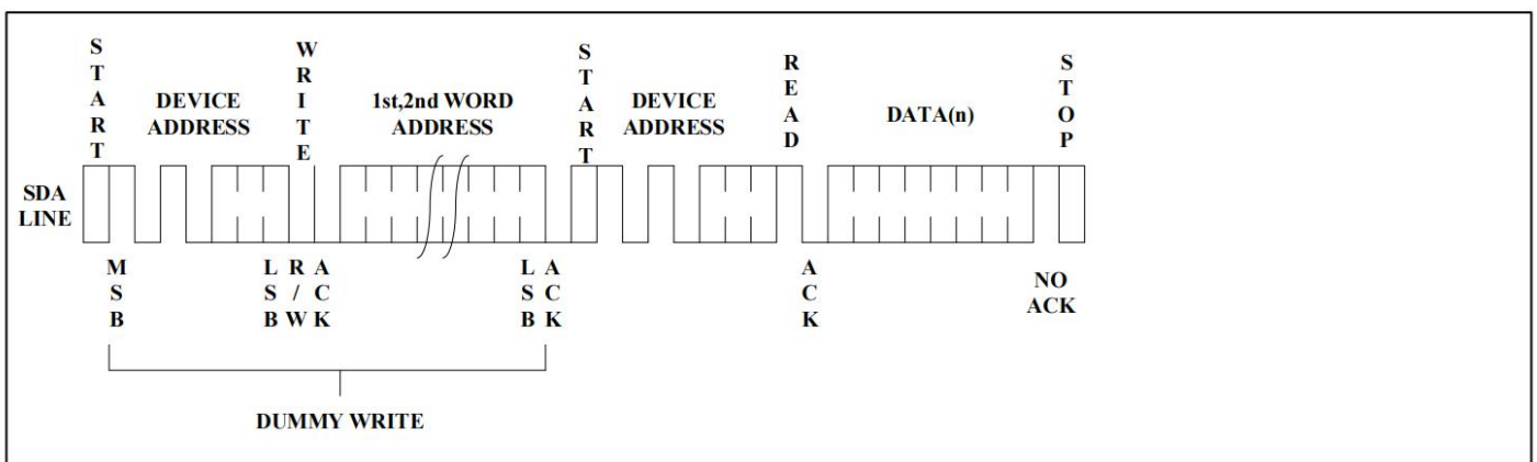
Figure 9. Random Read
