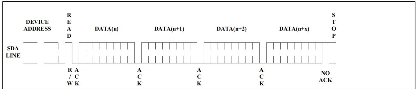
Figure 10. Sequential Read
