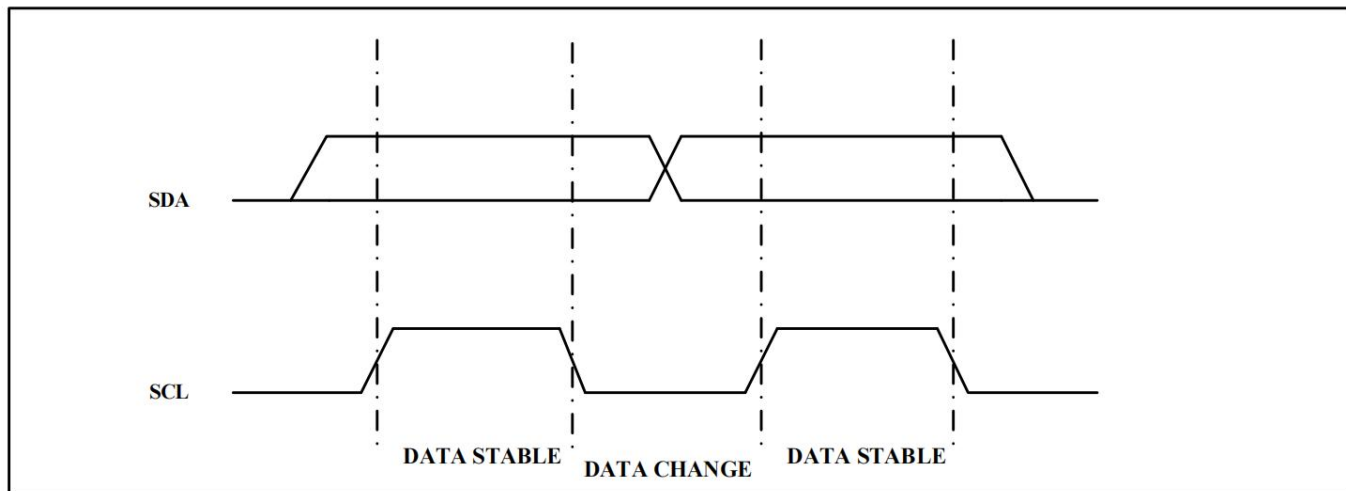
Figure 2. Data Validity
