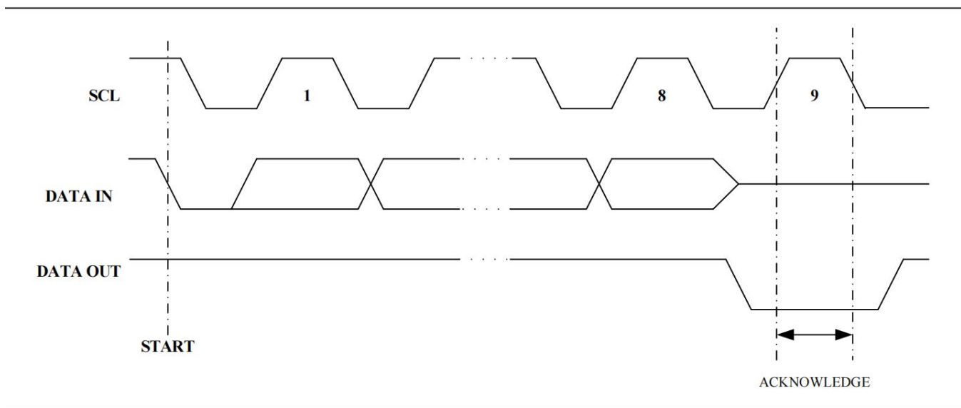
Figure 4. Output Acknowledge
