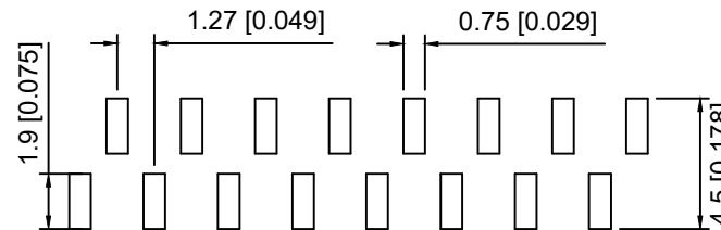
PCB LAYOUT (R2)
