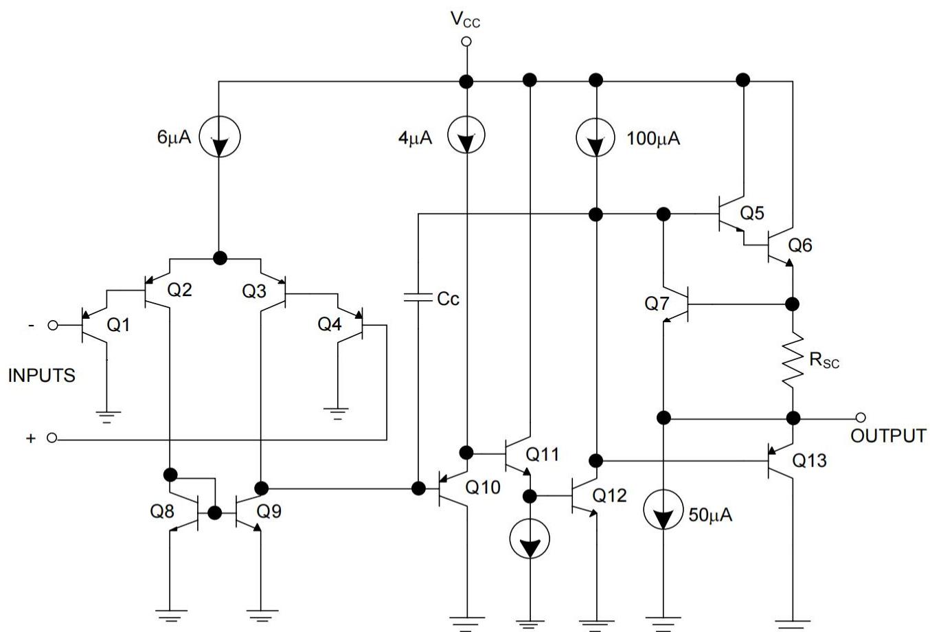
Functional Block Diagram of LM2902Q/LM2902AQ/LM2904Q/LM2904AQ (Each Amplifier)
