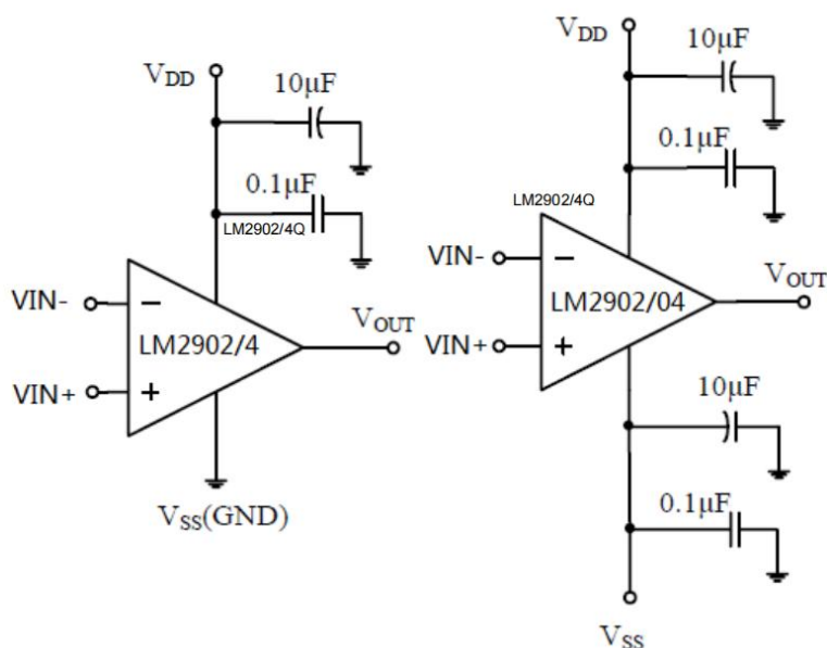
Amplifier with Bypass Capacitors
