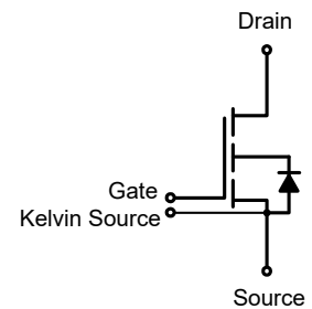
Schematic Symbol
