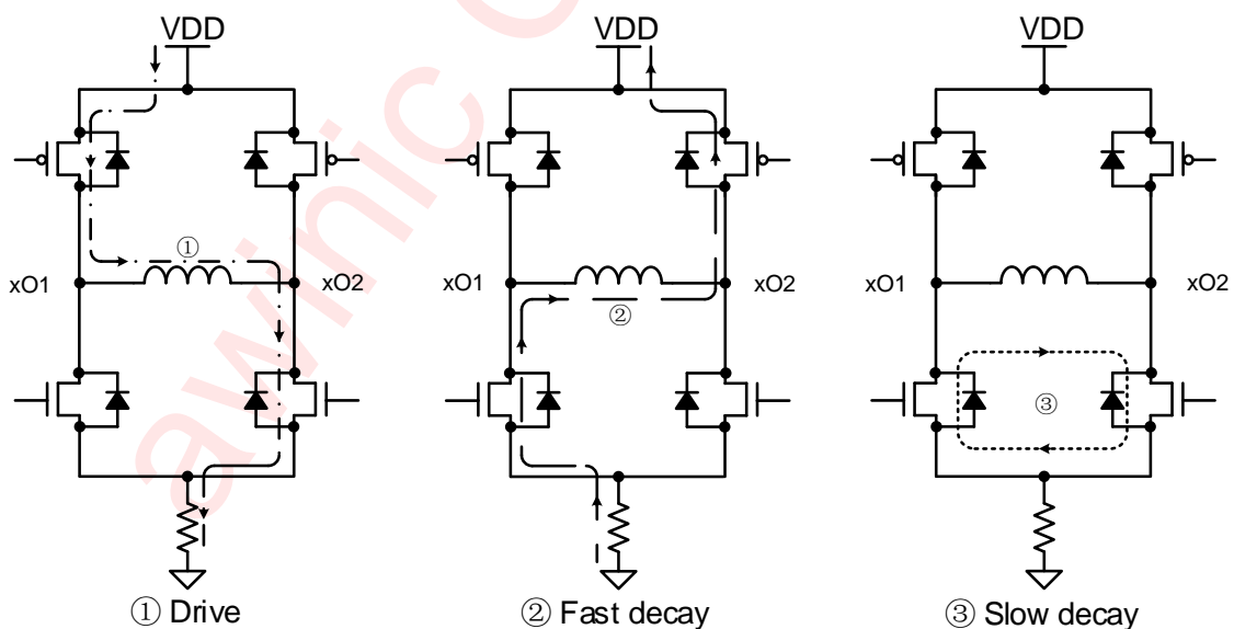
Figure 6 Decay Modes
