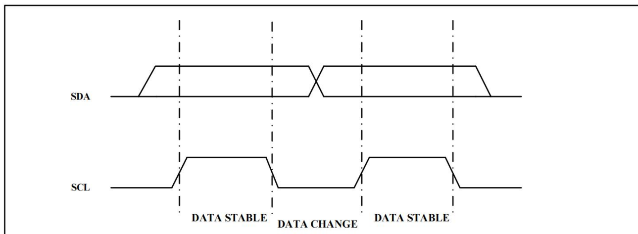
Figure 2. Data Validity
