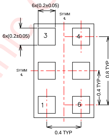
BOTTOM VIEW
