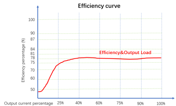
Figure 5: Efficiency VS Output Load (Nominal Voltage Input)
