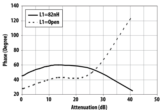
Figure 54. Phase vs Attenuation with and without External L1 at 900MHz
