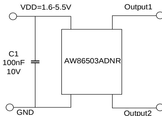
Figure 1 Typical Application Circuit of AW86503ADNR
