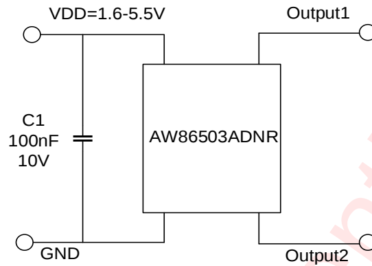
Figure 6 The Application Circuit of AW86503ADNR
