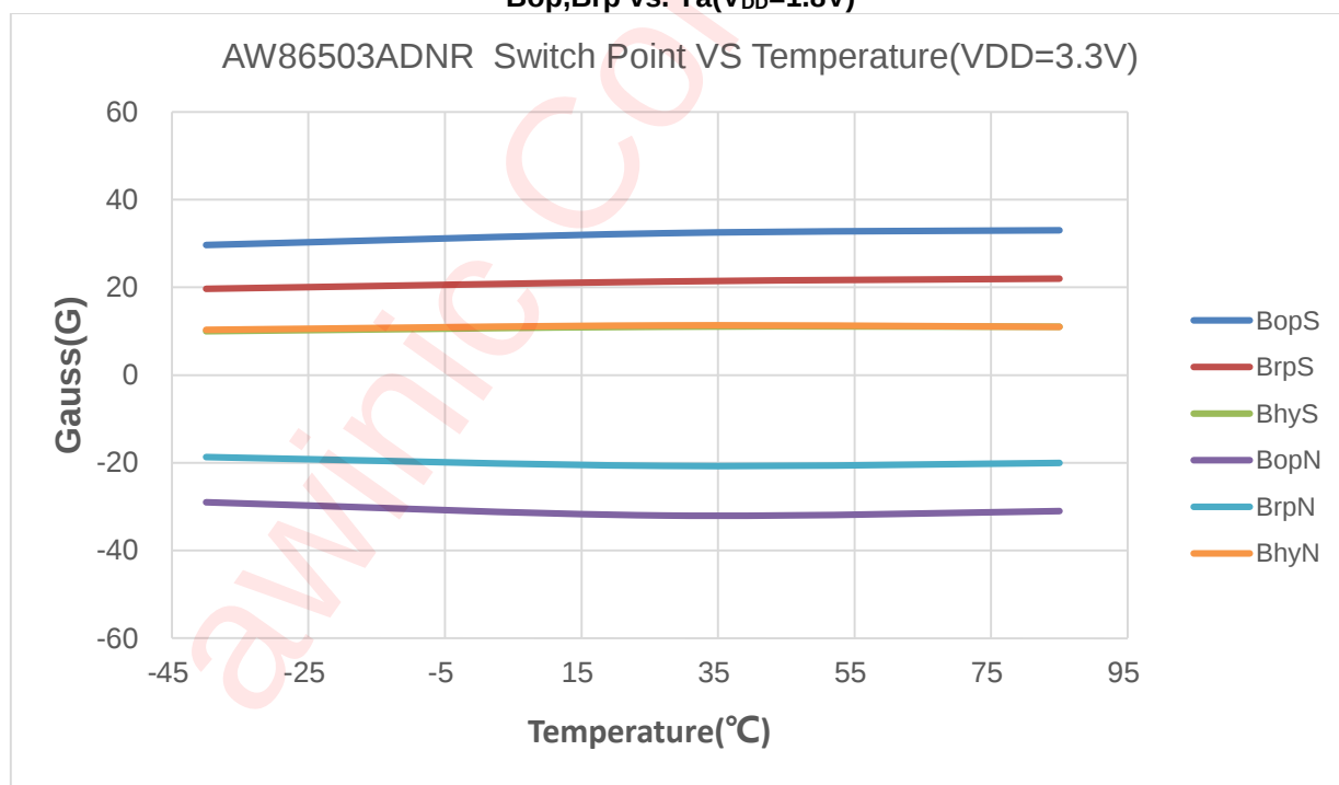
Figure 5 The Typical Characteristics of AW86503ADNR
