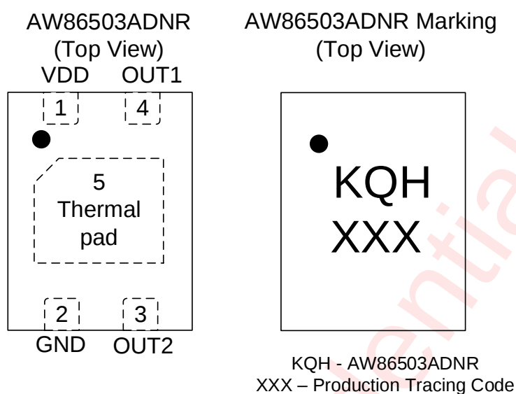
Figure 2 Pin Configuration and Top Mark
