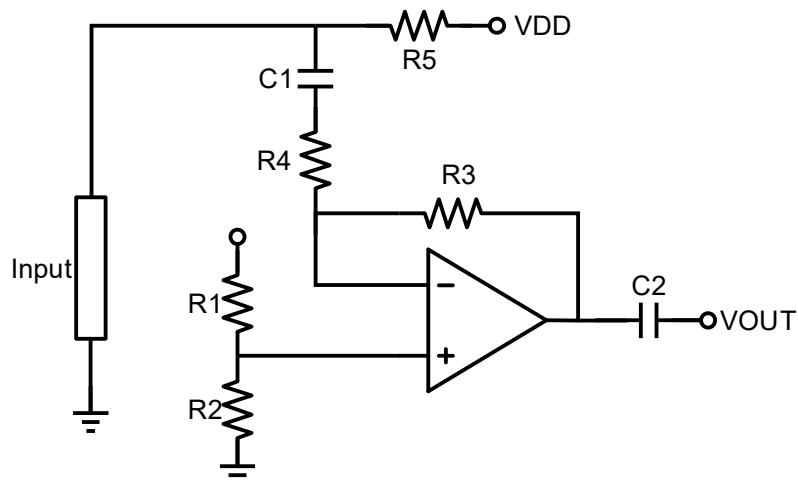
Figure 1. Typical Application
