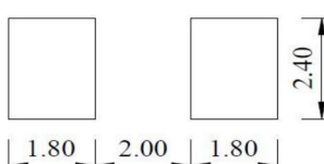
Recommended Solder Pattern
