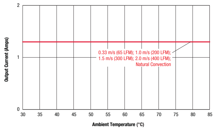
Maximum Current Temperature Derating at sea level VIN = 12V (air flow from Pin 1 to Pin 2 on PCB)
