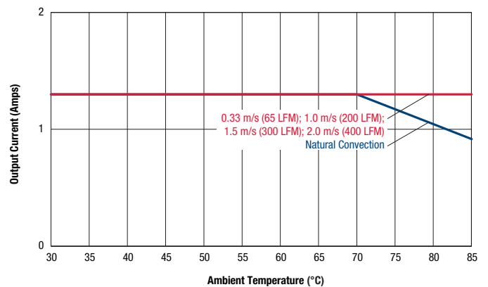
Maximum Current Temperature Derating at sea level VIN = 36V (air flow from Pin 1 to Pin 2 on PCB)
