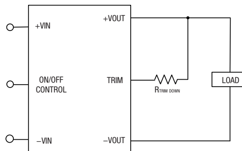
Figure 3. Trim adjustments to decrease Output Voltage using a Fixed Resistor
