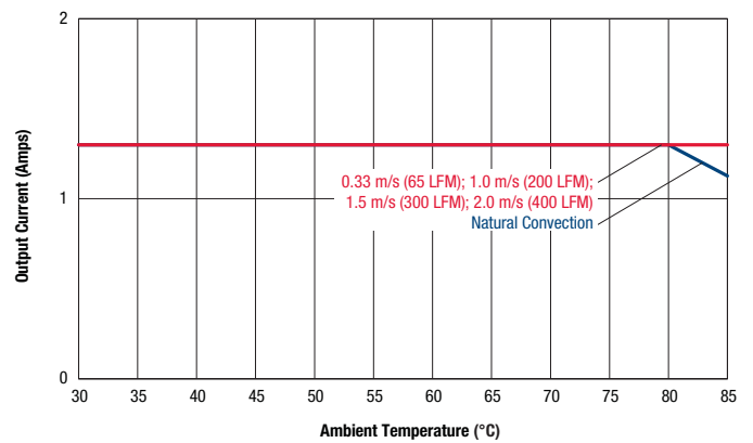
Maximum Current Temperature Derating at sea level VIN = 24V (air flow from Pin 1 to Pin 2 on PCB)
