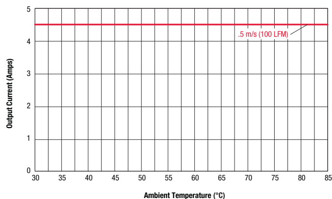
Maximum Current Temperature Derating at sea level VIN = 36V (air flow from Pin J1 to Pin J2 on PCB)
