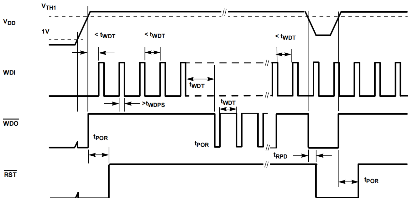
FIGURE 5. WATCHDOG TIMING DIAGRAM
