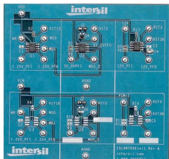
FIGURE 15. ISL88705EVAL1
