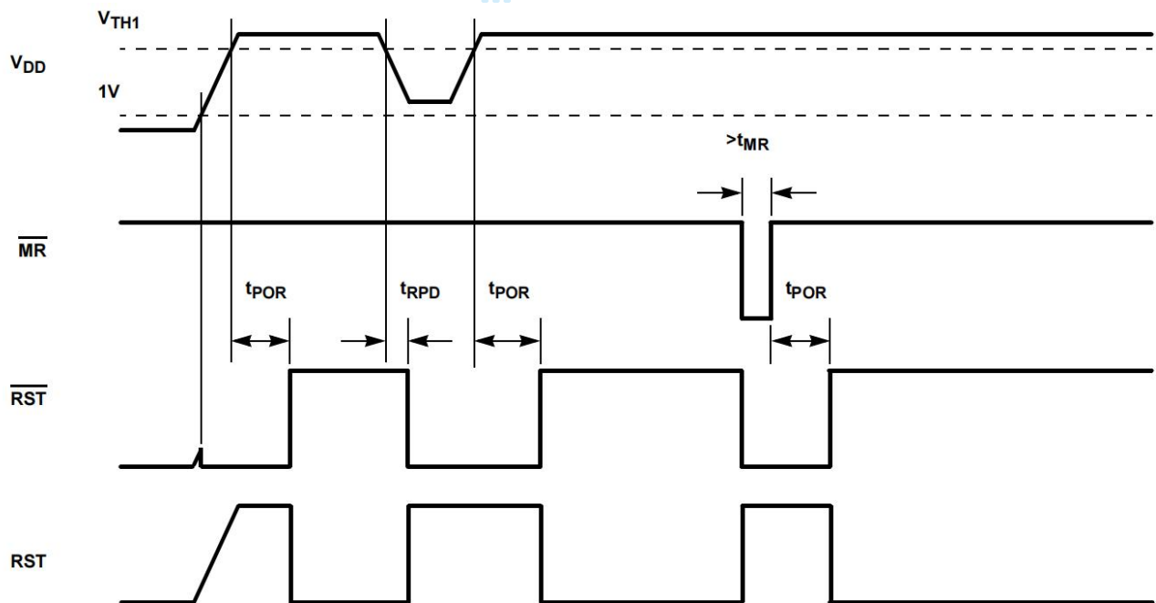
FIGURE 1. POWER-SUPPLY MONITORING TIMING DIAGRAM (WDI TRI-STATèD)
