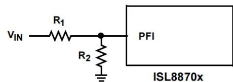
FIGURE 2. CUSTOM V_{TH} WITH RESISTOR DIVIDER ON PFI
