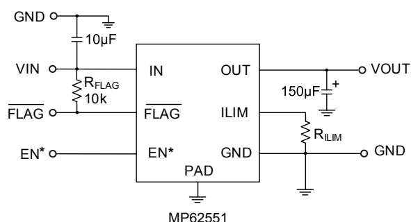
Figure 4—Application Circuit
