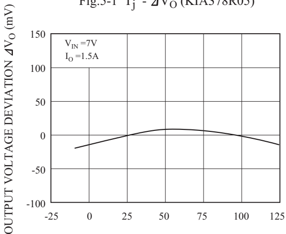
Fig.5-1 T_j - \Delta V_O (KIA378R05)
