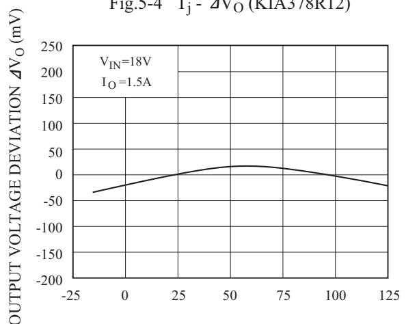
Fig.5-4 T_j - \Delta V_O (KIA378R12)
