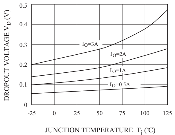
Fig.8 T_j - V_D
