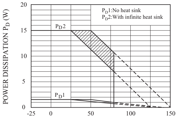
Fig.3 T_a - P_D
