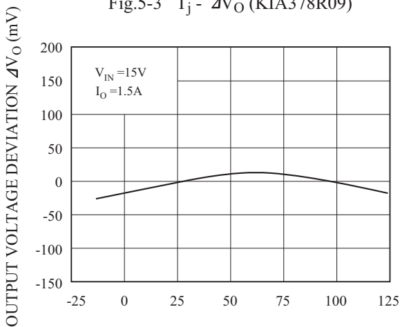
Fig.5-3 T_j - \Delta V_O (KIA378R09)
