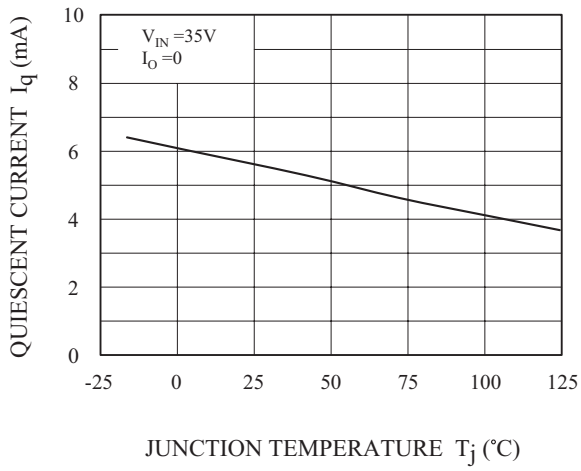
Fig.9 T_j - I_q
