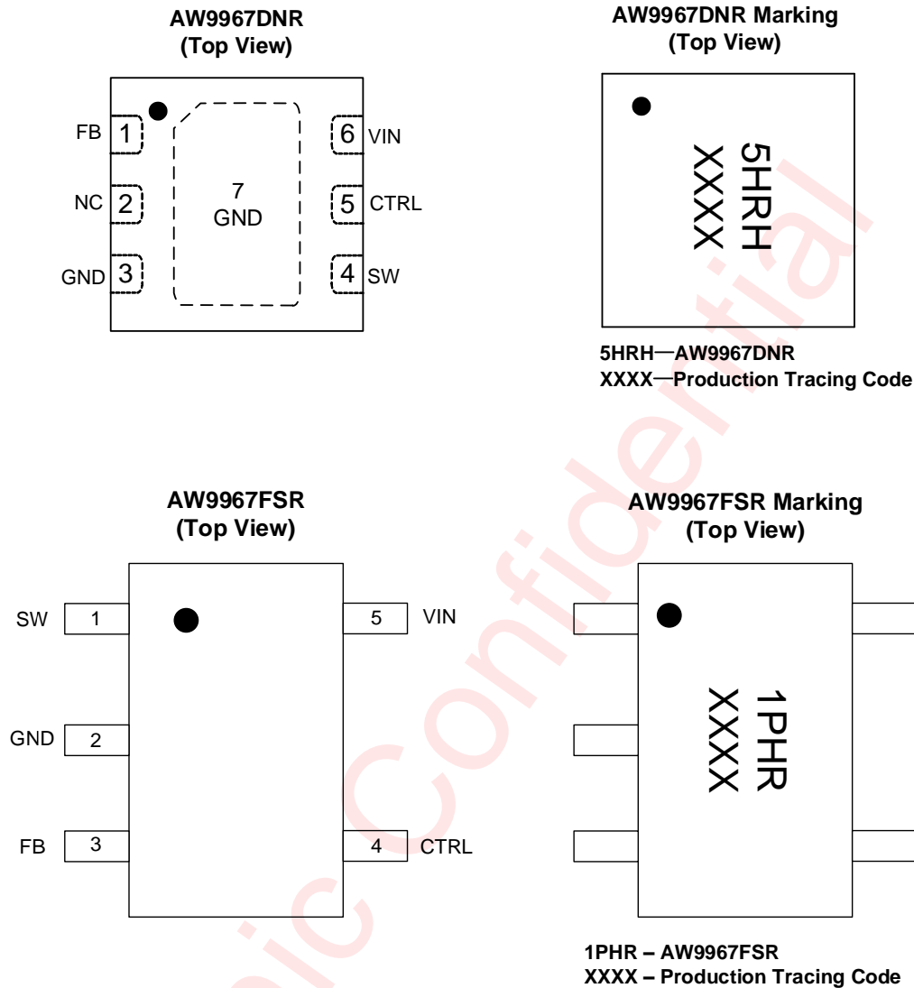
Figure 1 Pin Configuration and Top Mark
