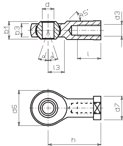
Single Knuckle Joint/DIN648 - DIN24335
