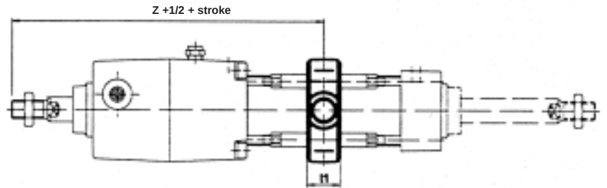
Trunnion Type
