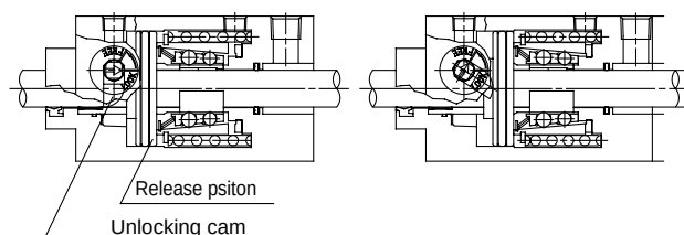
Locked condition
