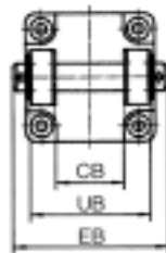
Rear single clevis C Rear double clevis D
