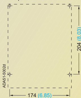
Drill pattern
