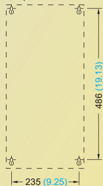
Drill pattern
