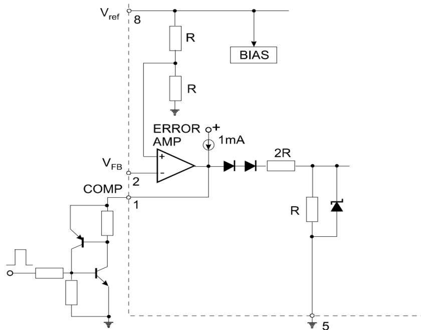
Figure 5. Latched Shutdown
