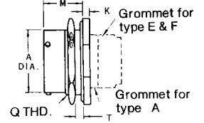
Crimp KPSE07/MS3124
