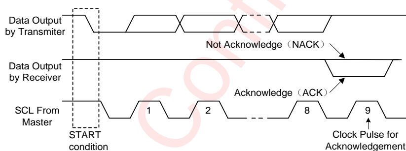
Figure 25 Acknowledgement Diagram
