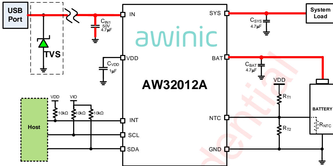
Figure 1 Typical Application Circuit of AW32012A
