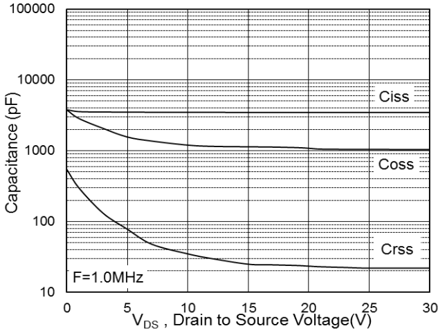
Fig.7 Capacitance
