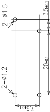
DRILLING DIAGRAM(2/1) (BOTTOM VIEW)
