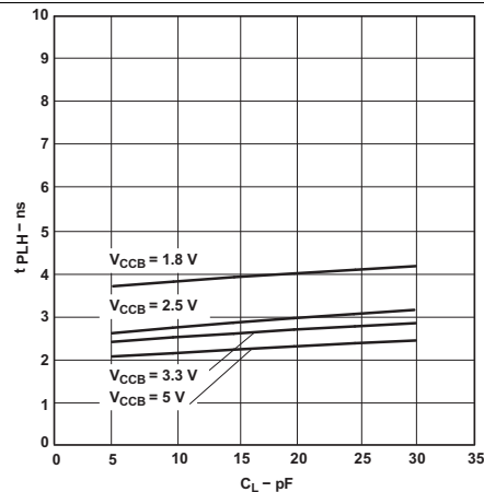
Figure 16. Typical Propagation Delay (B to A) vs Load Capacitance
