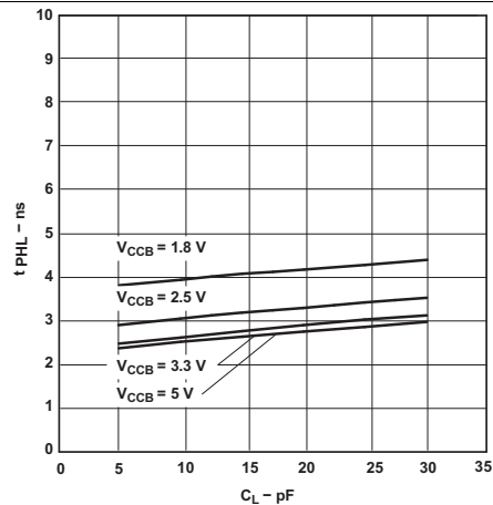
Figure 11. Typical Propagation Delay (B to A) vs Load Capacitance
