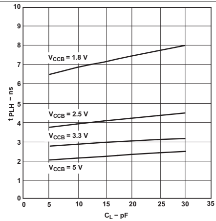
Figure 14. Typical Propagation Delay (A to B) vs Load Capacitance
