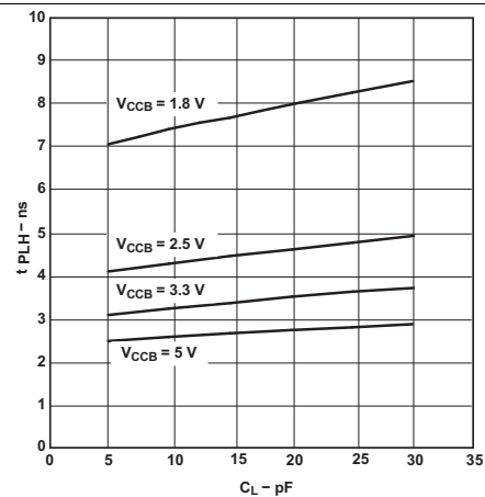
Figure 10. Typical Propagation Delay (A to B) vs Load Capacitance
