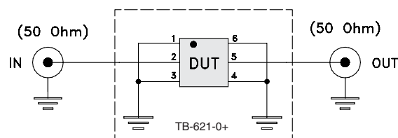
Fig 1. Block diagram of Test Circuit used for characterization, Test board TB-621-0+ Conditions: Attenuation, VSWR: Pin=-10 dBm
