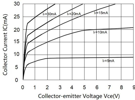
Fig.3 Collector Current vs. Collector-emitter Voltage
