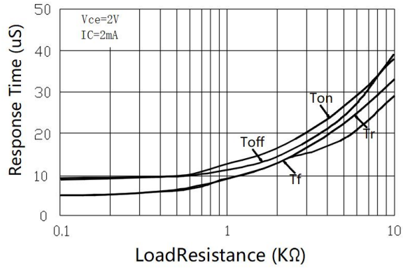
Fig.7 Response Time vs. Load Resistance
