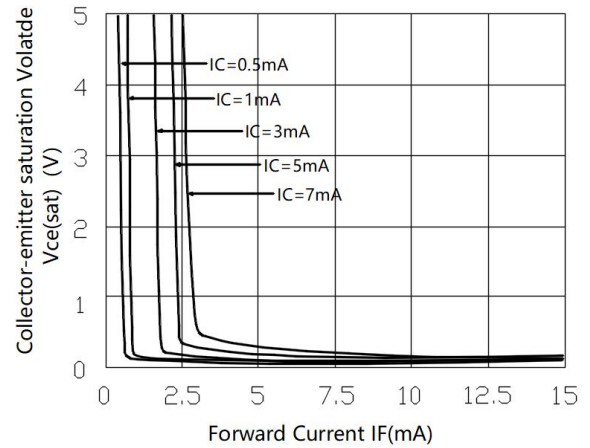
Fig.8 Collect-emitter Saturation Voltage vs. Forward Current
