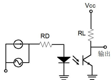
Fig.10 Test Circuit for Response Time
