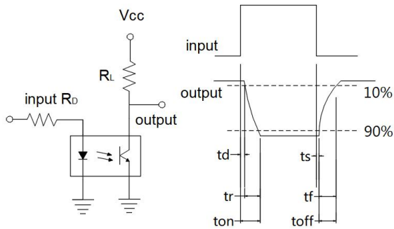
Fig.9 Switching Time Test Circuit & Wave forms
