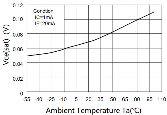
Fig.5 Collector-emitter Saturation Voltage vs. Ambient Temperature
