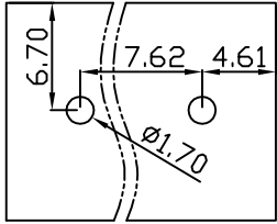
PCB Layout
