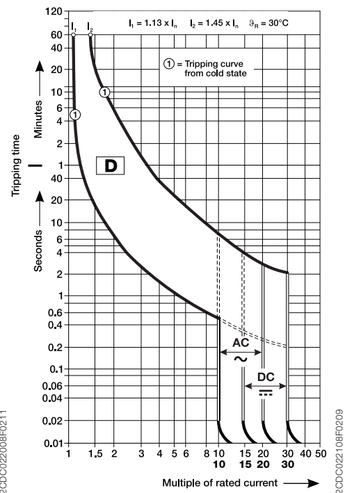
D characteristic
