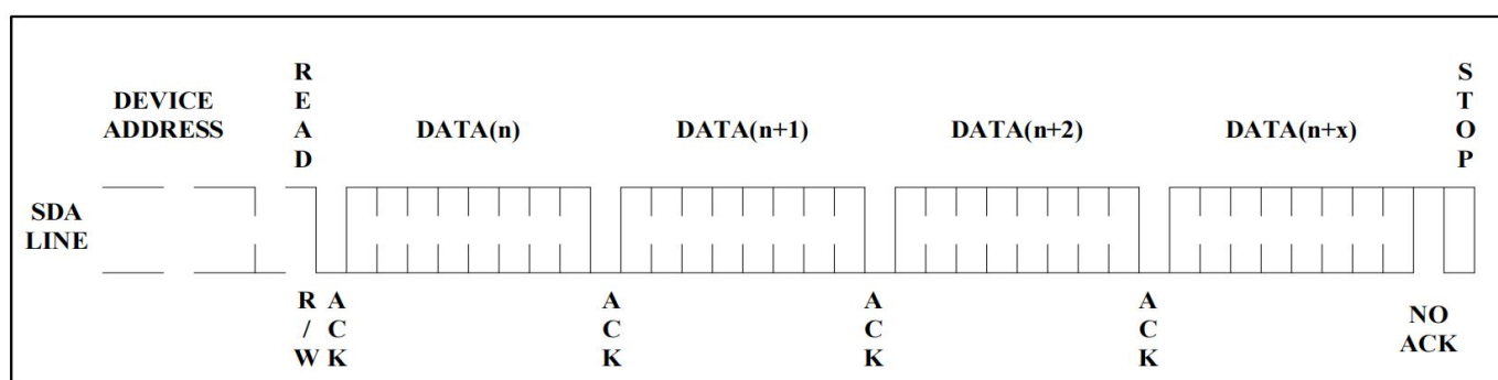
Figure 10. Sequential Read
