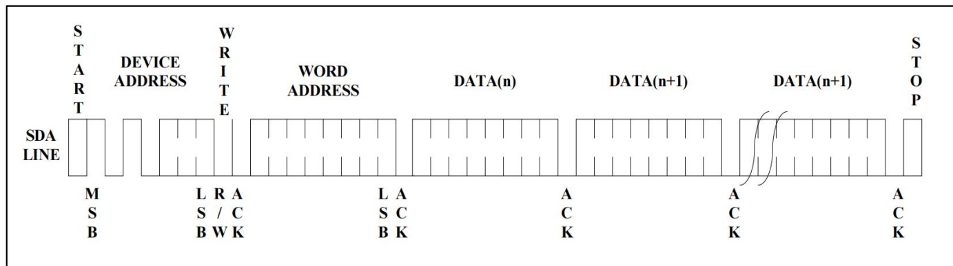
Figure 7. Page Write
