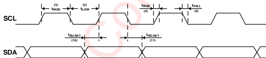
Figure 7 SCL and SDA timing relationships in the data transmission process
