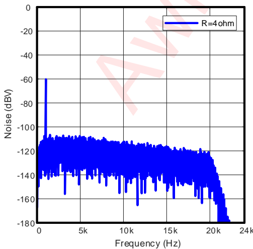
Noise FFT With -60dB Output
