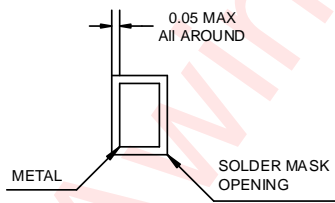
NON-SOLDER MASK DEFINED
