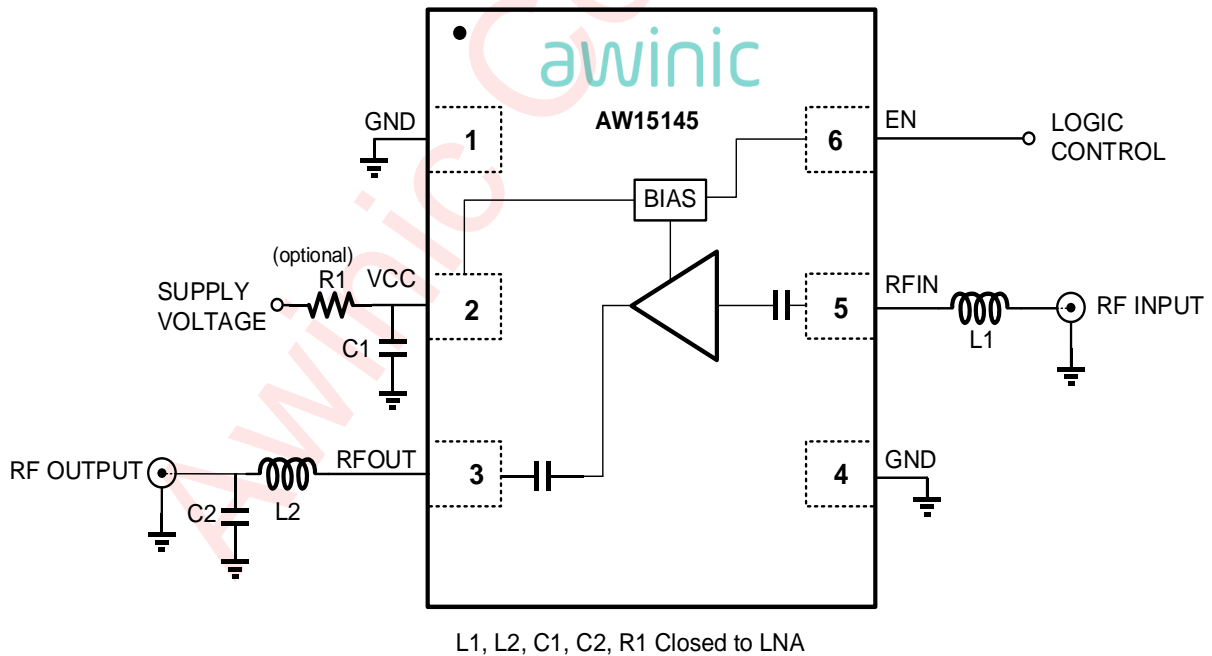
Figure 1(a) Typical Application Circuit of AW15145 for GPS L1
