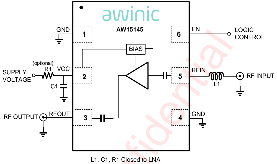
Figure 1(a) Typical Application Circuit of AW15145 for GPS L1
