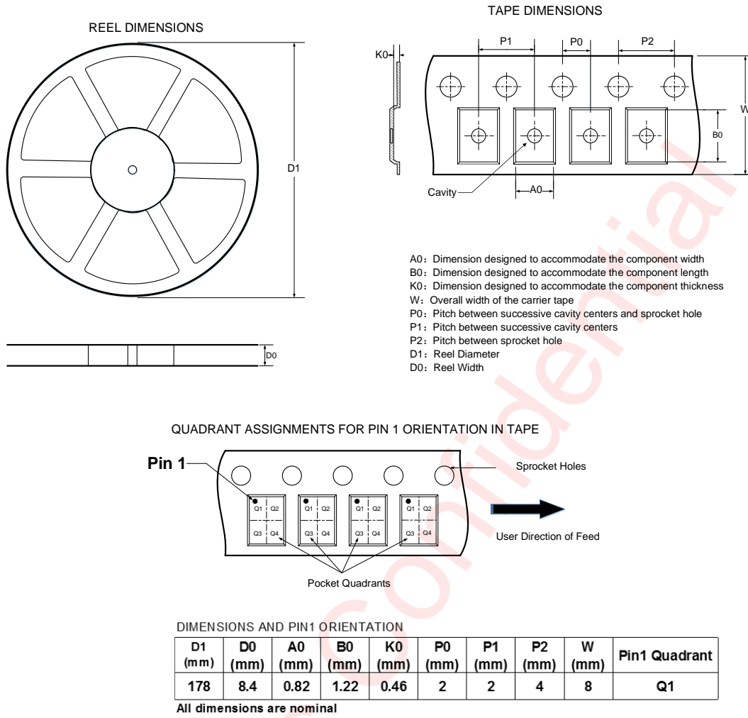
Figure 13 AW15145DNRA Tape & Reel Description
