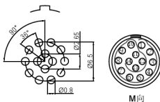
Pcb plate opening size (PCB板开孔尺寸)
