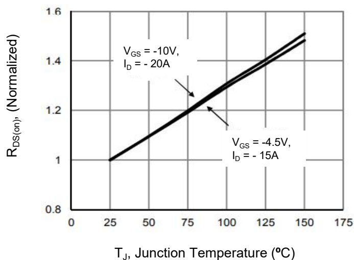
Figure 7. Drain-Source On-Resistance
