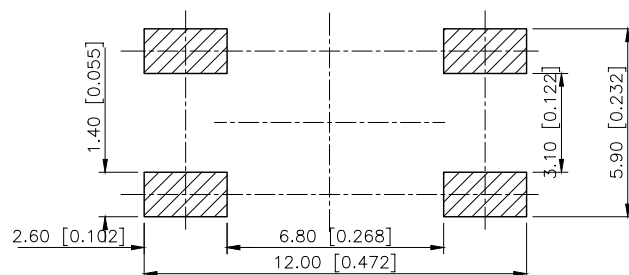
P.C.B MOUNTING HOLES
