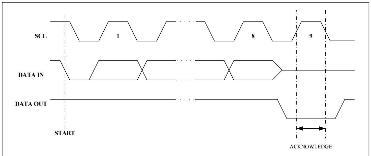
Figure 4. Output Acknowledge
