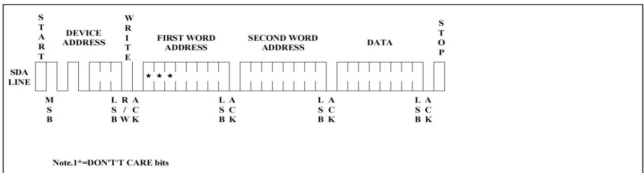
Figure 7. Byte Write
