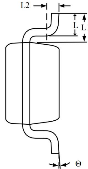
SIDE VIEW
