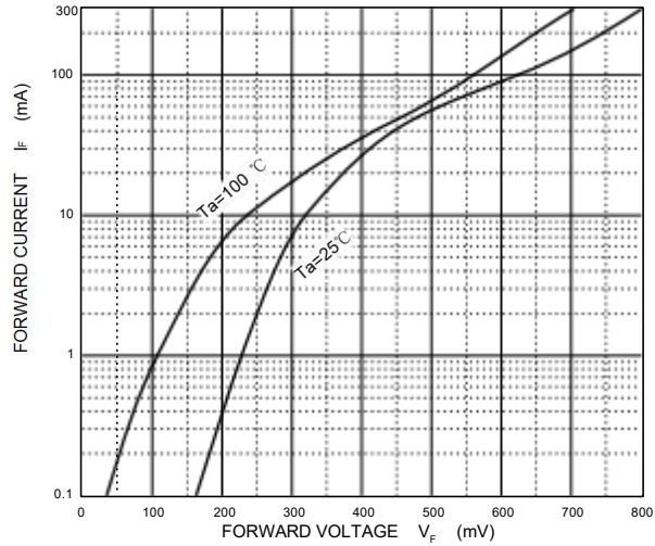
Forward Characteristics
