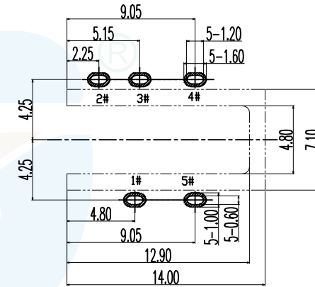
PCB LAYOUT (TOP VIEW) TOLERANCE: ±0.05
