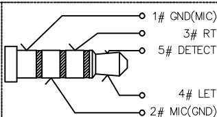
Ø3.50mm 4 POLE PLUG SCHEMATIC
