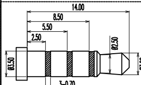
Ø3.50mm 4 POLE PLUG DETAIL
