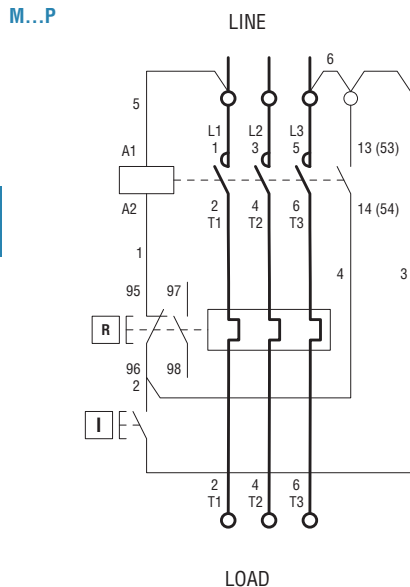
Diagram 1 - Incorporated button control
