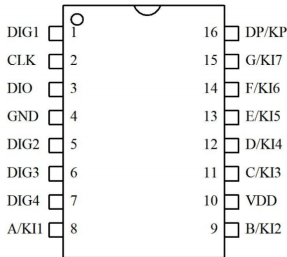
GM1650 SOP16
