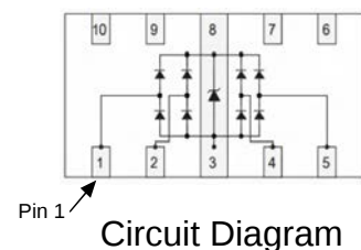
DFN2510-10L (SGP2510-8P)
