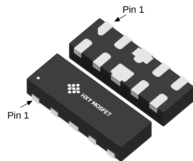
DFN2510-10L (SGP2510-8P)
