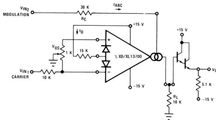
Figure 23. Amplitude Modulator
