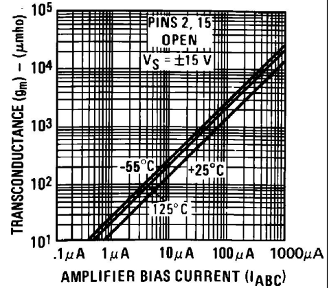
Figure 8. Transconductance
