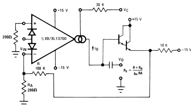
Figure 25. AGC Amplifier
