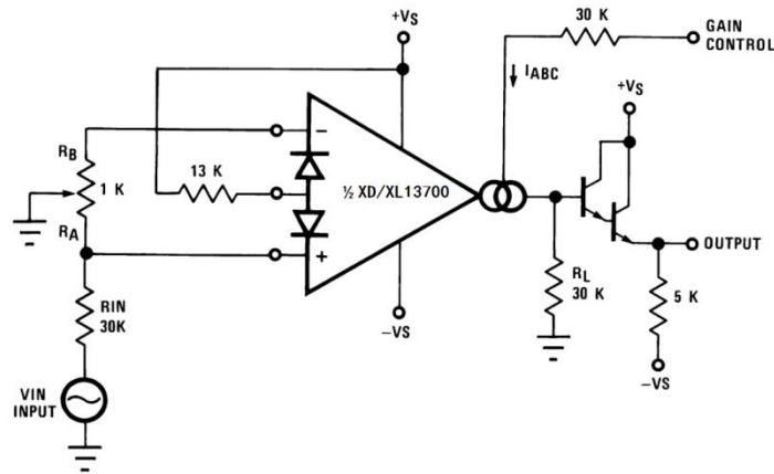
Figure 20. Voltage-Controlled Amplifier
