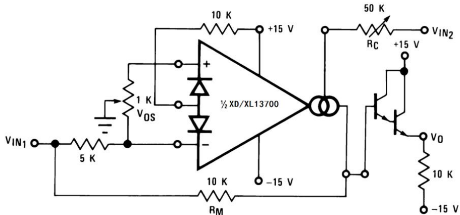
Figure 23. Amplitude Modulator
