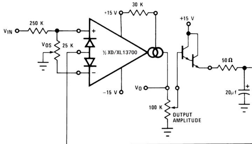
Figure 25. AGC Amplifier
