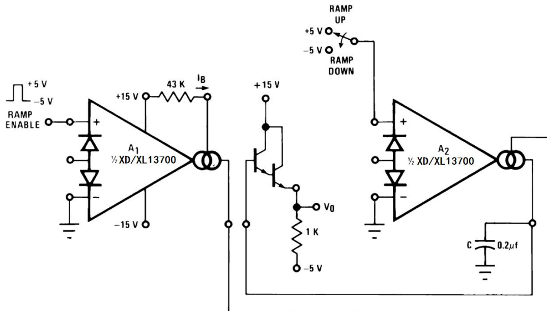
Figure 43. Sample-Hold Circuit
