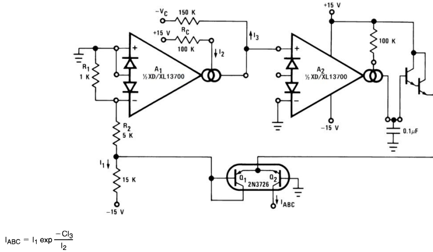
Figure 48. Logarithmic Current Source
