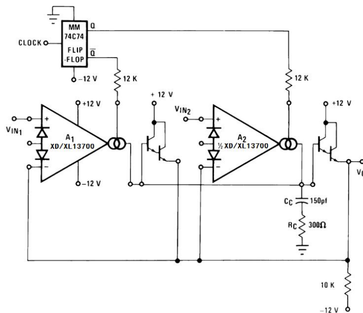
Figure 38. Multiplexer
