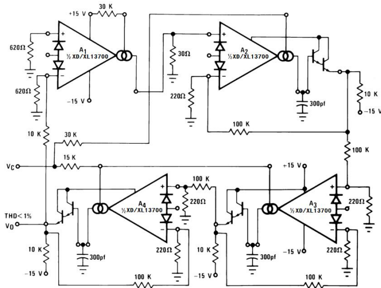
Figure 35. Sinusoidal VCO
