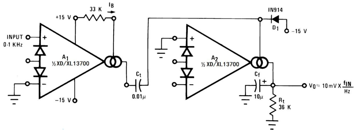
Figure 41. Tachometer
