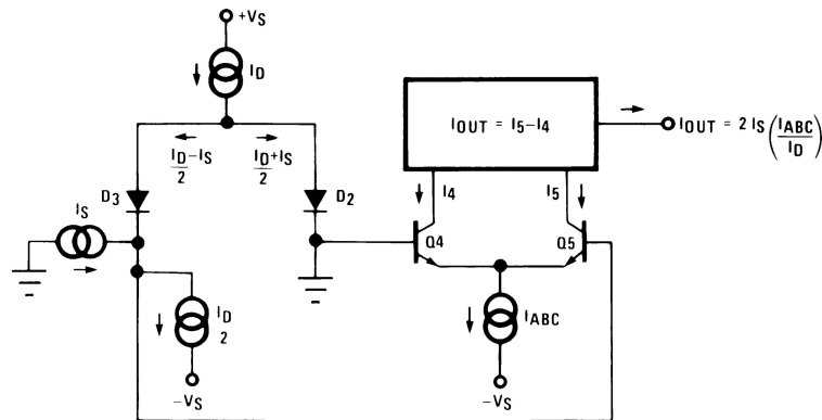
Figure 19. Linearizing Diodes
