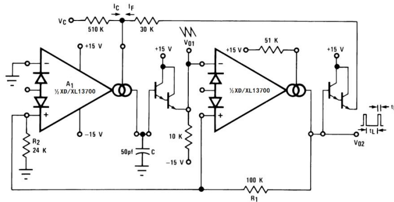
Figure 33. Triangular/Square-Wave VCO
