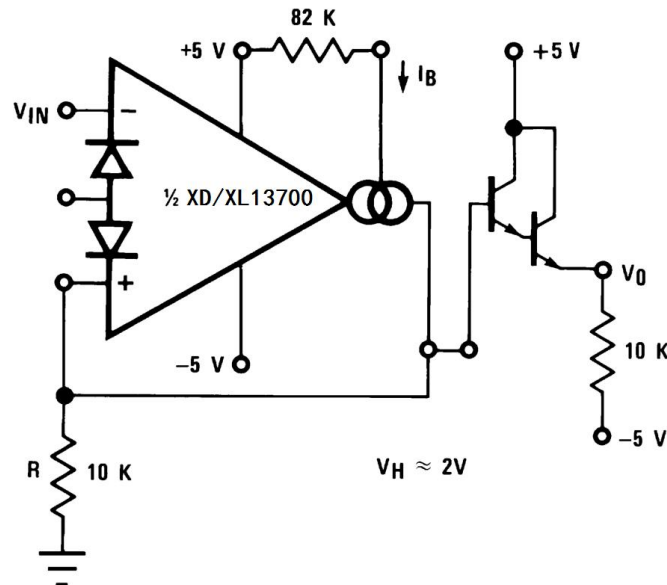
Figure 40. Schmitt Trigger
