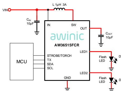
Typical Application Circuit of AW36515
