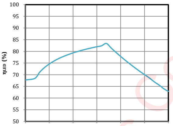
I_{LED} = 1.5A V_{LED} = 3.5V f_{SW} = 2MHz Flash LED Efficiency vs Input Voltage
