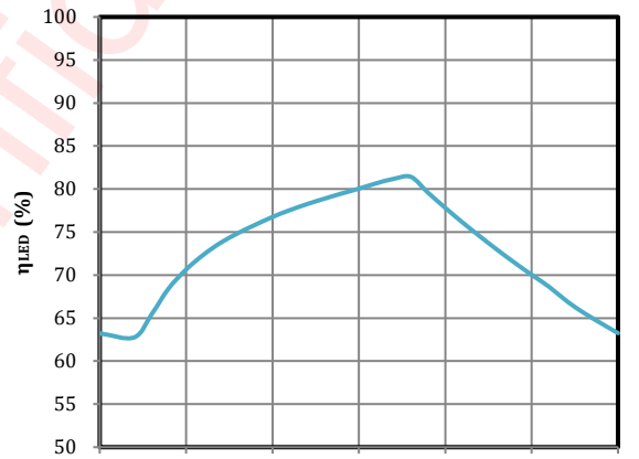
I_{LED} = 1.5A V_{LED} = 3.5V f_{SW} = 4MHz Flash LED Efficiency vs Input Voltage
