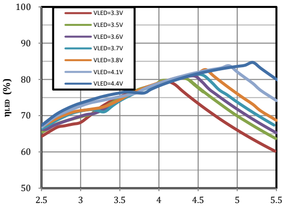
I_{LED} = 2.0A f_{SW} = 2MHz Flash LED Efficiency vs Input Voltage
