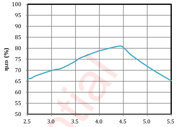
I_{LED} = 2.0A V_{LED} = 3.6V f_{SW} = 2MHz Flash LED Efficiency vs Input Voltage
