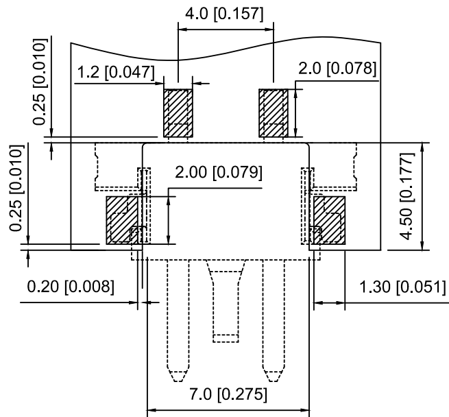
PCB LAYOUT
