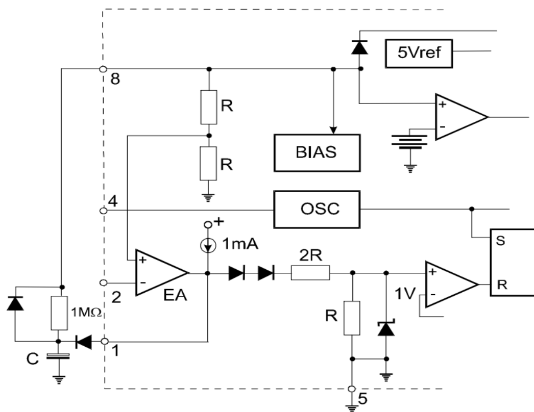
Figure 8. Soft-Start Circuit
