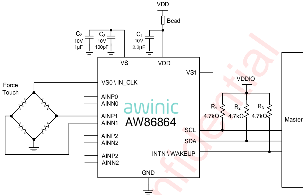
Figure 1 AW86864 Typical Application Circuit
