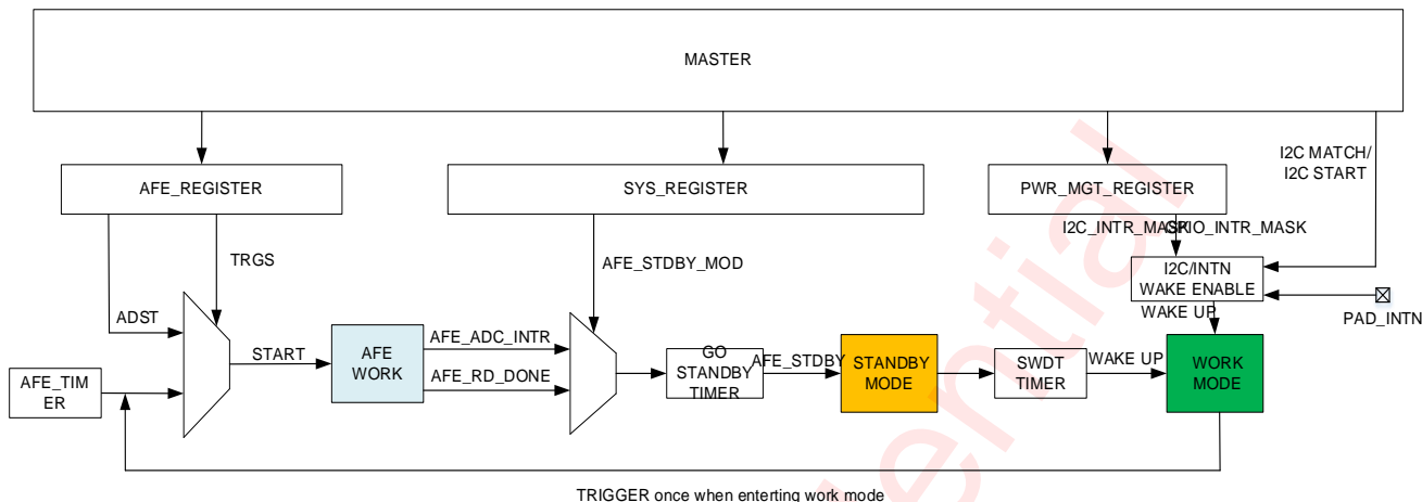
Figure 10 System Workflow
