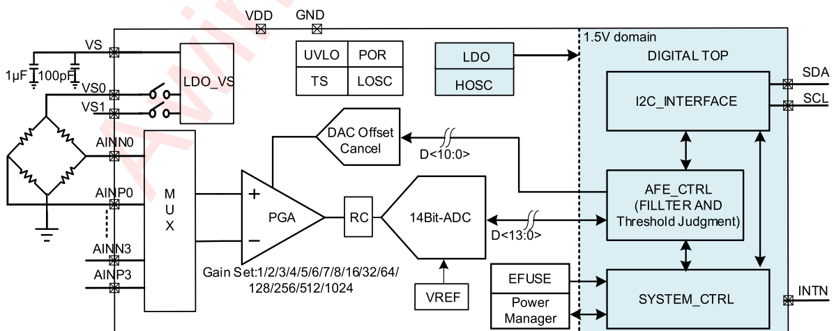
Figure 3 AW86864 Function Block Diagram
