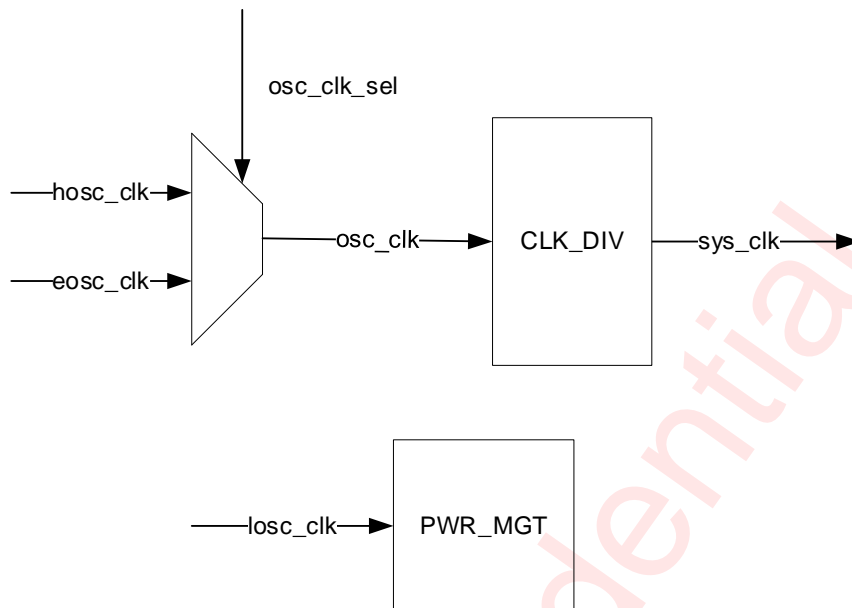
Figure 9 Clock Tree
