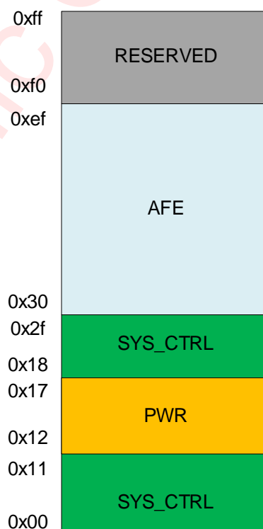
Figure 12 AW86864 Register Address Distribution
