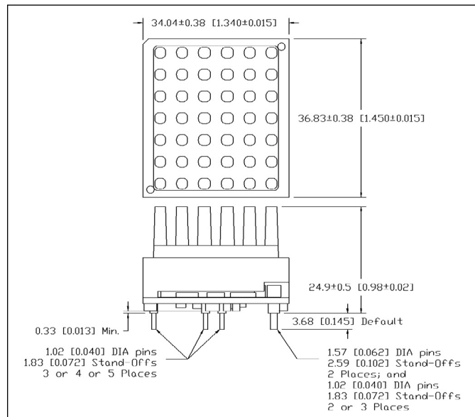
Heatsink - xFx-R Series (i7C4W)
