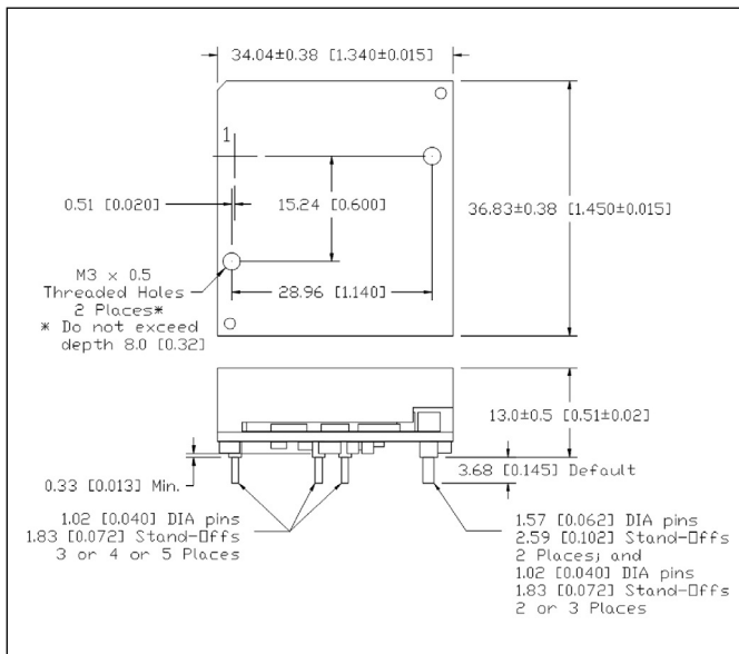
Baseplate - xCx-R Series (i7C4W)
