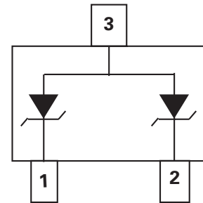
Circuit diagram
